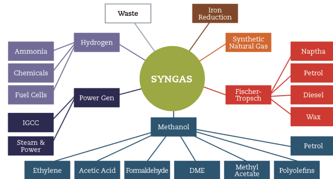
Figure 2--Gasification converts carbon-based materials into syngas. Syngas can be converted into methanol. Methanol
