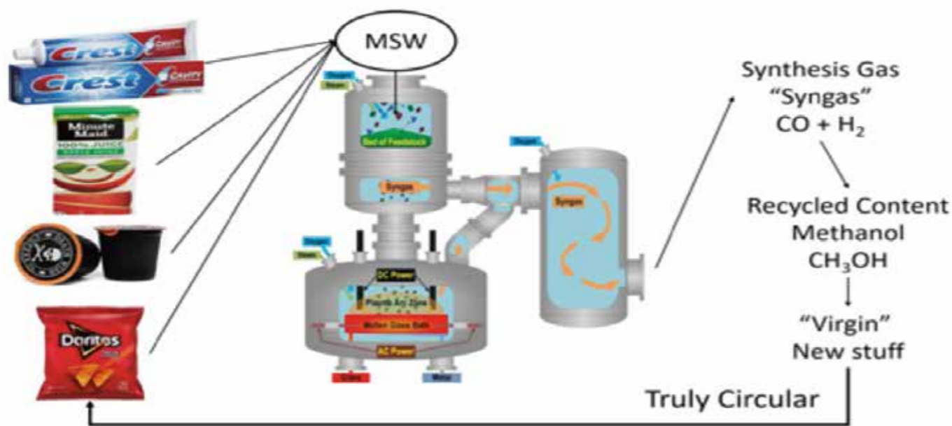
Figure 1: Plasma Assisted Gasification and Vitrification (PAG/V) process converts mixed waste into syngas.
